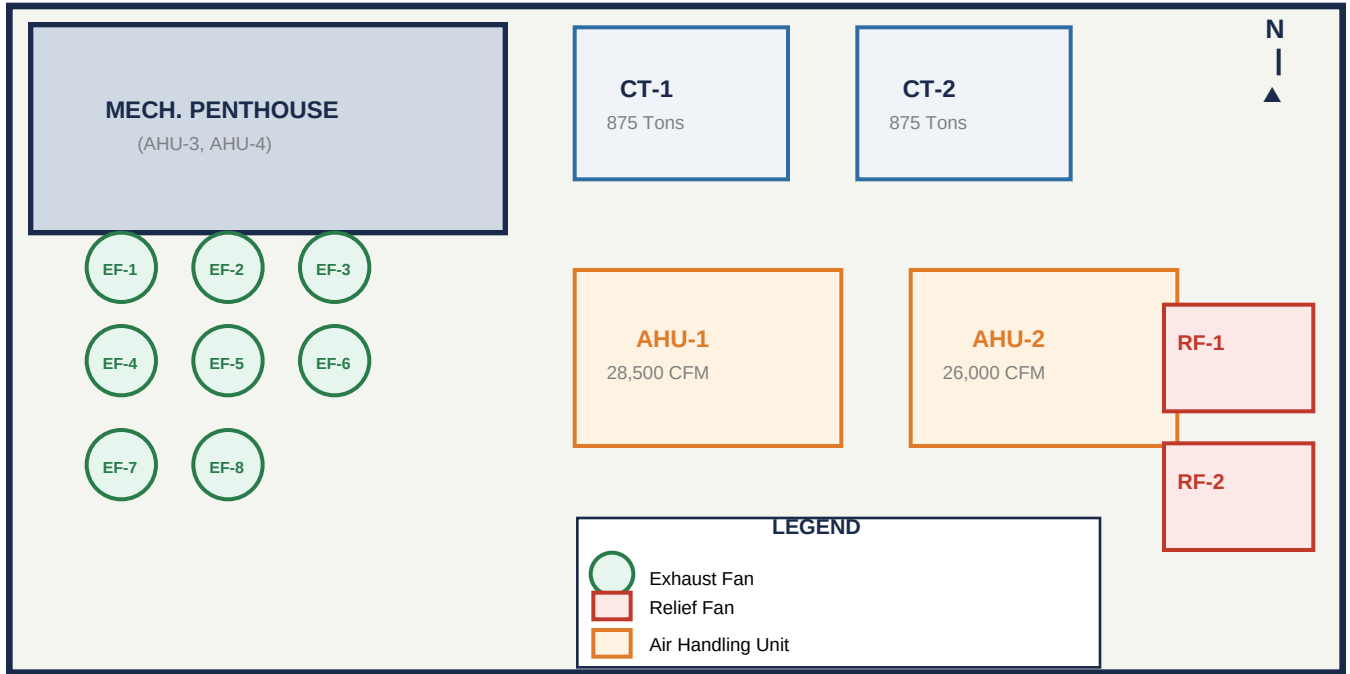
Figure 5 — Rooftop Mechanical Equipment Plan (Schematic — Not to Scale)
